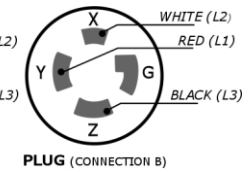
PLUG (CONNECTION B)
