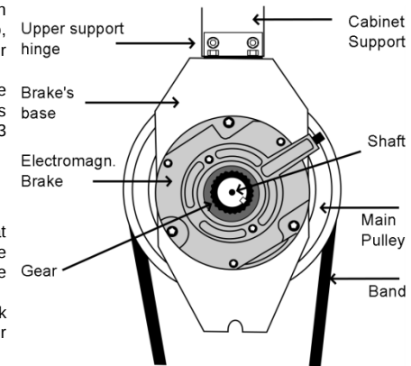
FIG. A1 ELECTROMAGNETIC BRAKE
