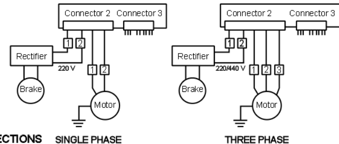
FIG. A2 CONNECTIONS SINGLE PHASE
